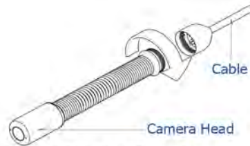
Figure 8. Assembly/Disassembly Camera
