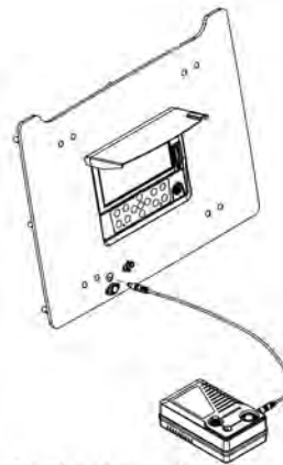
Figure 10. Install power cable
