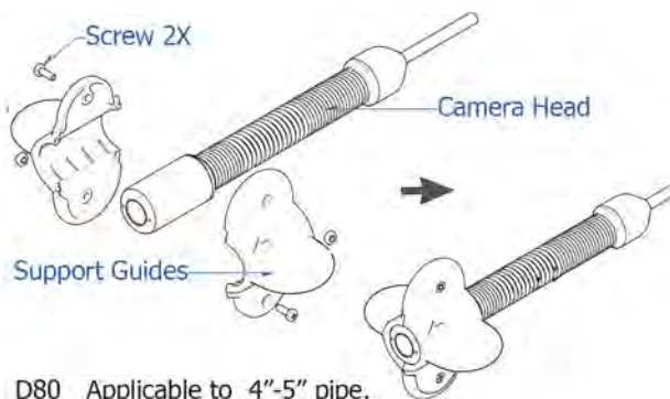
Figure 12. Install 80 Support Guides
